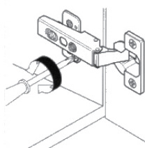
Height adjustment
